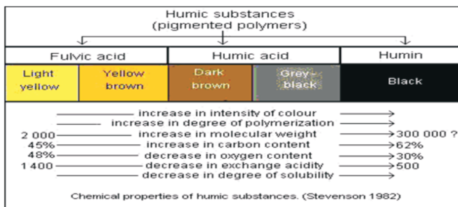
Figure 1. Chemical nature of humic substances (Stevenson,1982)
